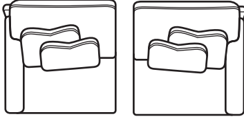
709-031 LSF Chair 709-030 RSF Chair 40 W 41 D 38 H 26 AH 20 SH
